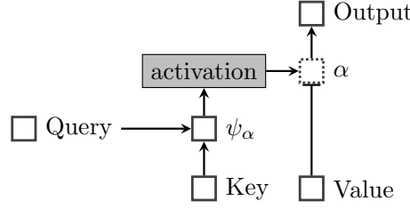
Figure 18.6: A general view of neural attention. The dotted box indicates that each \alpha_{m \rightarrow n} can be viewed as a gate on value n .
