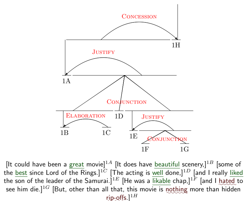
Figure 16.5: A rhetorical structure theory analysis of a short movie review, adapted from Voll and Taboada (2007). Positive and negative sentiment words are underlined, indicating RST’s potential utility in document-level sentiment analysis.
